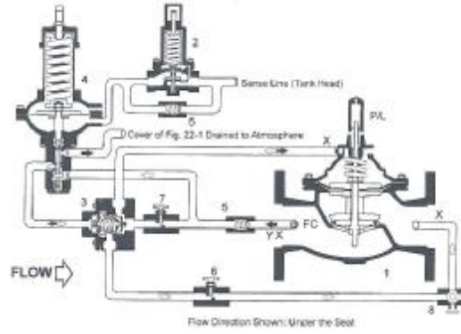
WATTS ACV-127-2 蓄水塔進水出水水位控制閥
