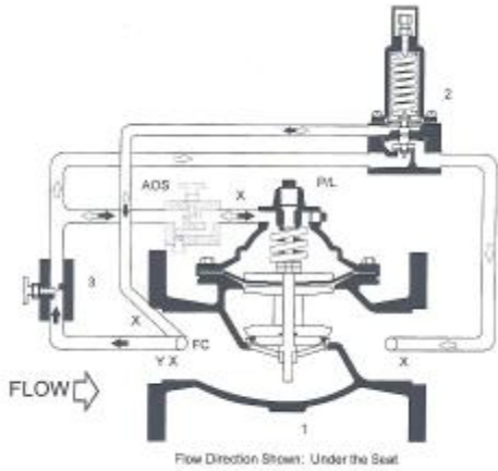
WATTS ACV-116 持壓閥
